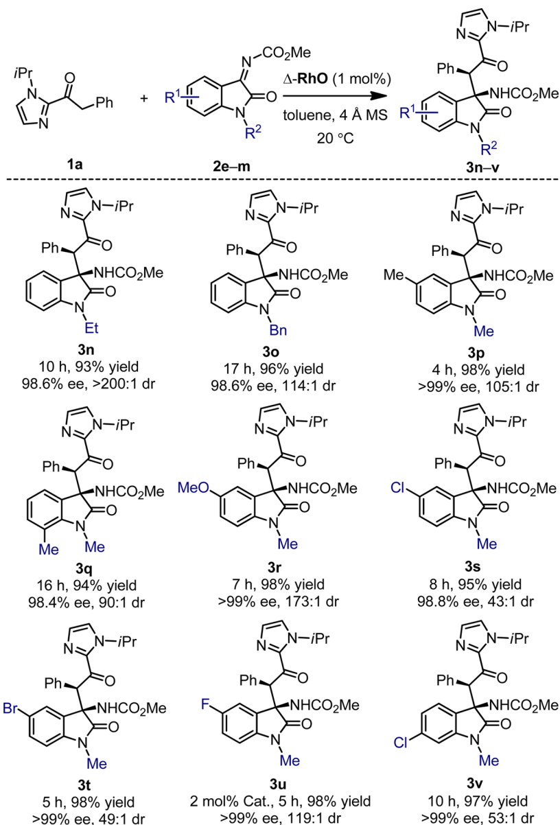
Scheme 2. Scope Regarding Isatin-Derived Ketimines
