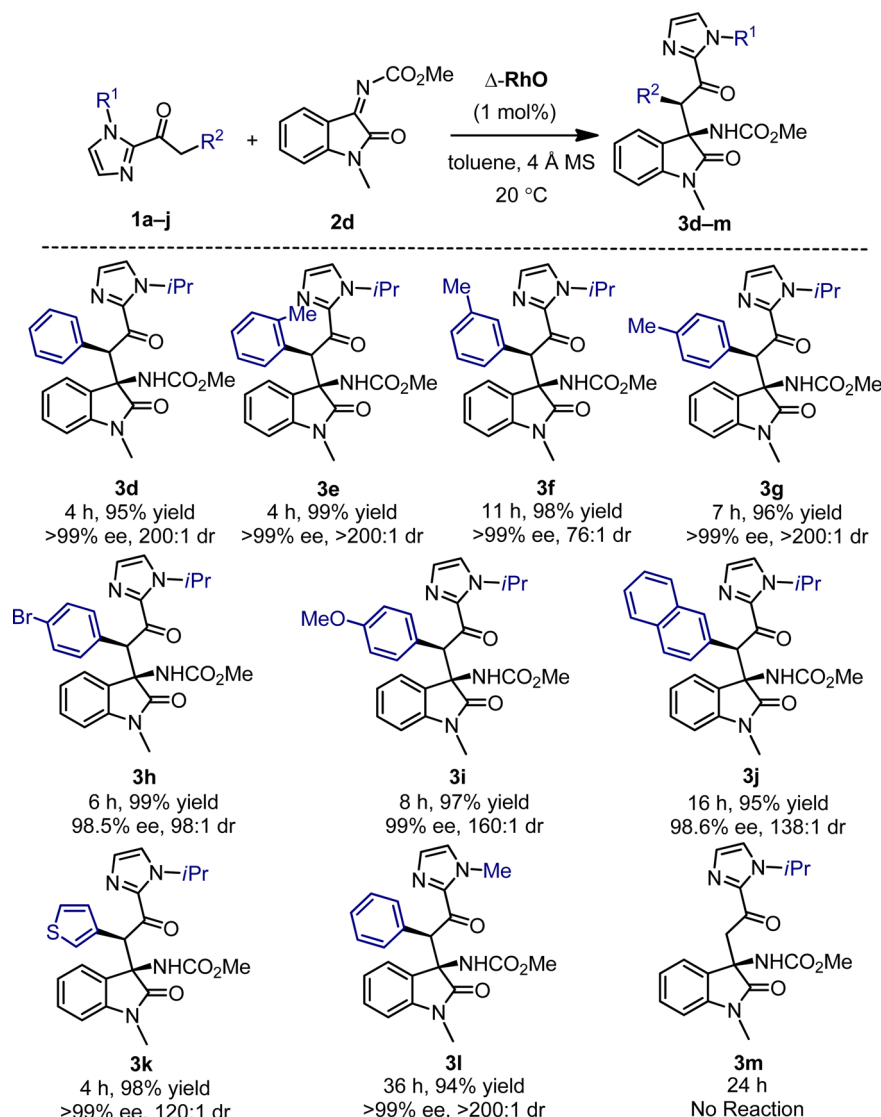
Scheme 1. Scope Regarding 2-Acyl Imidazoles
