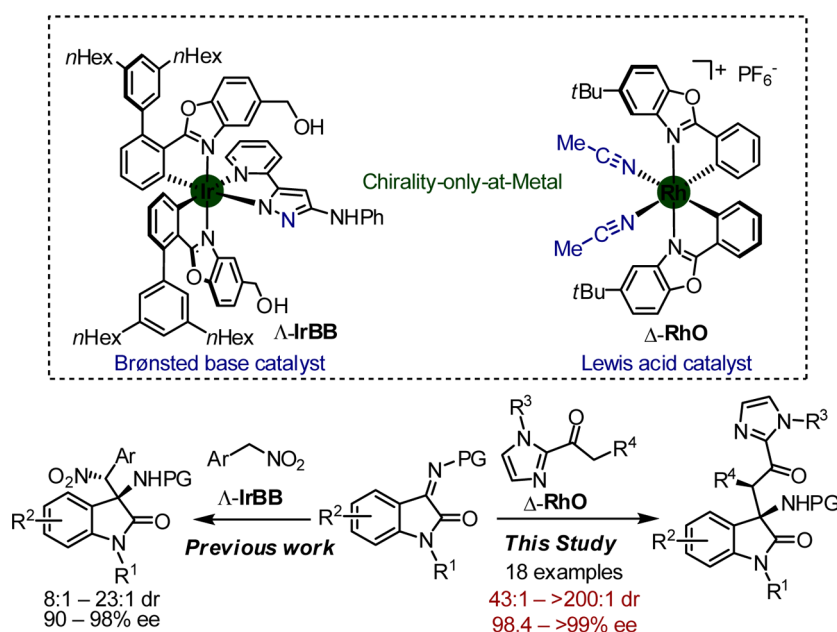
Figure 1. Previous work and this study on stereoselective synthesis of chiral 3,3-disubstituted oxindoles by chiral-at-metal catalysts.
